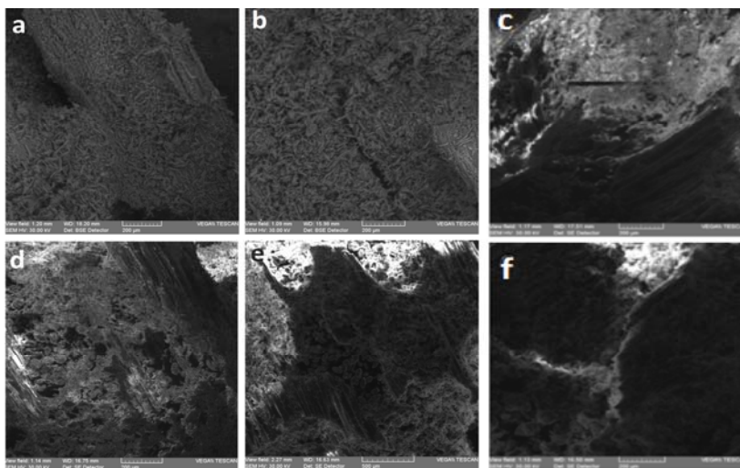
Fig. 3. SEM microscopy of the six samples before the consolidation treatment: a - Sample taken from P1 (200X, BSE); b - Sample taken from P2 (200X, BSE); c - Sample taken from P3 (200X, SE); d - Sample taken from P4 (200X, SE); e - Sample taken from P5 (100X, SE); f - Sample taken from P6 (200X, SE);
