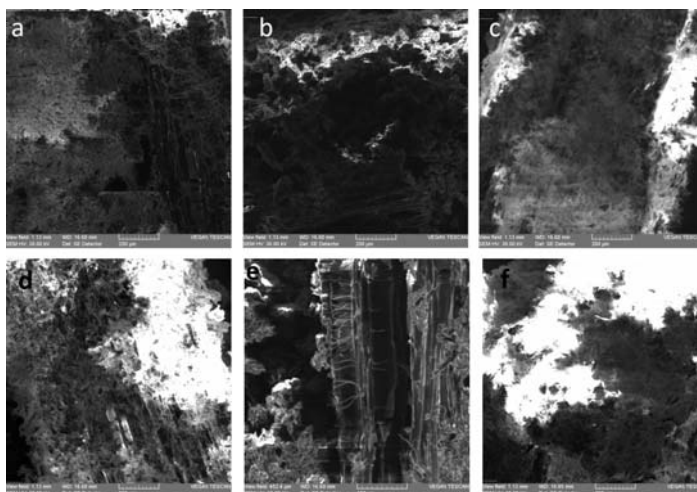
Fig. 5. SEM microscopy of the six samples after the consolidation treatment: a - Sample taken from P1 (200X, SE); b - Sample taken from P2 (100X, SE); c - Sample taken from P3 (200X, SE); d - Sample taken from P4 (200X, BSE); e - Sample taken from P5 (500X, BSE); f - Sample taken from P6 (200X, SE);
