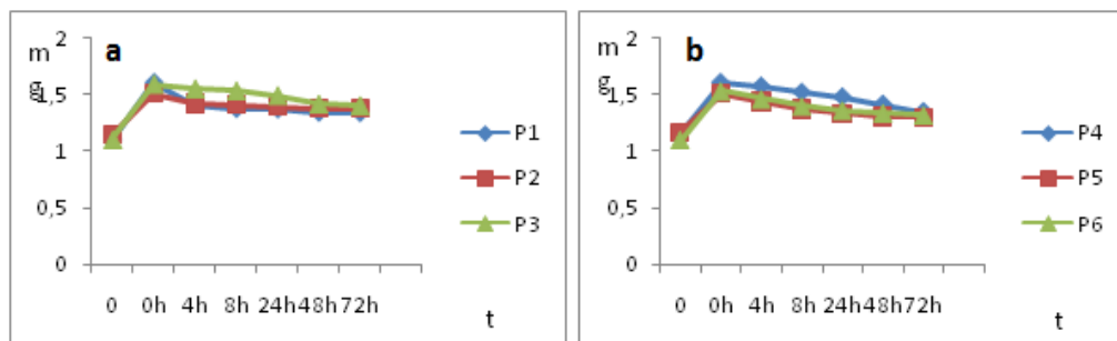
Fig. 7. Weight measurements of the six wood samples: a - Weight measurements on the oak-tree samples P1, P2 and P3; b - Weight measurements on the lime-tree samples P4, P5 and P6;
