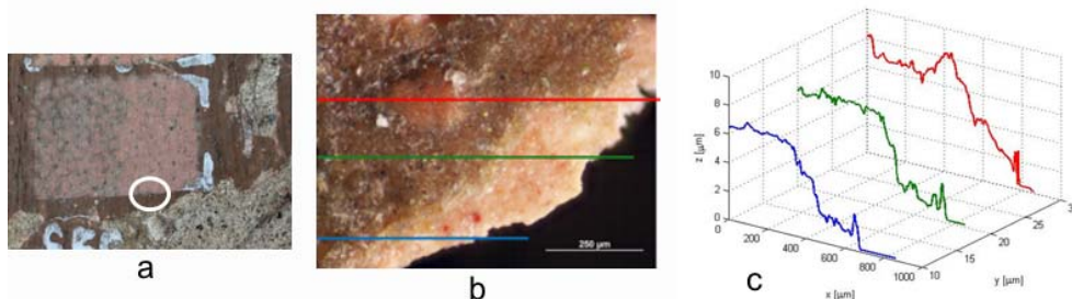
Fig. 6. (a) Detail of the SFR laser cleaned/not cleaned area; (b) Microscope image obtained by EDF module and lines reference for the profiles extraction; (c) 3D representation of the profiles.
